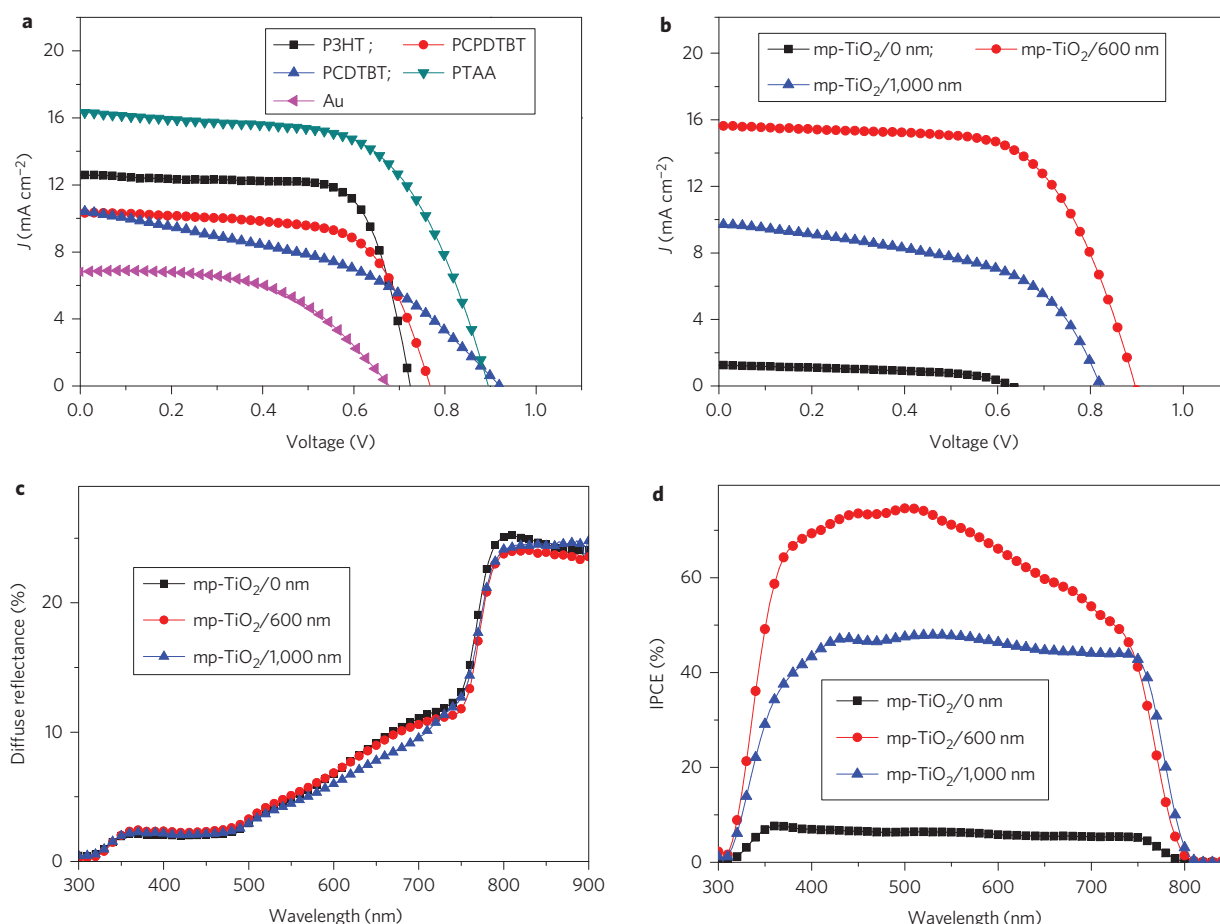
Figure 2 | J-V , diffuse reflectance and IPCE characteristics. a , J-V curves of inorganic-organic hybrid heterojunction solar cells with different hole-transporting layers ( \text{mp-TiO}_2 = 1 \mu\text{m} ). b , J-V curves of inorganic-organic hybrid heterojunction solar cells with different thicknesses of \text{mp-TiO}_2 film. c , Diffuse reflectance spectra of \text{FTO}/\text{bl-TiO}_2/\text{mp-TiO}_2/\text{CH}_3\text{NH}_3\text{PbI}_3/\text{Au} cells with different thicknesses of \text{mp-TiO}_2 film. d , IPCE spectra of inorganic-organic hybrid heterojunction solar cells with different thicknesses of \text{mp-TiO}_2 film.
