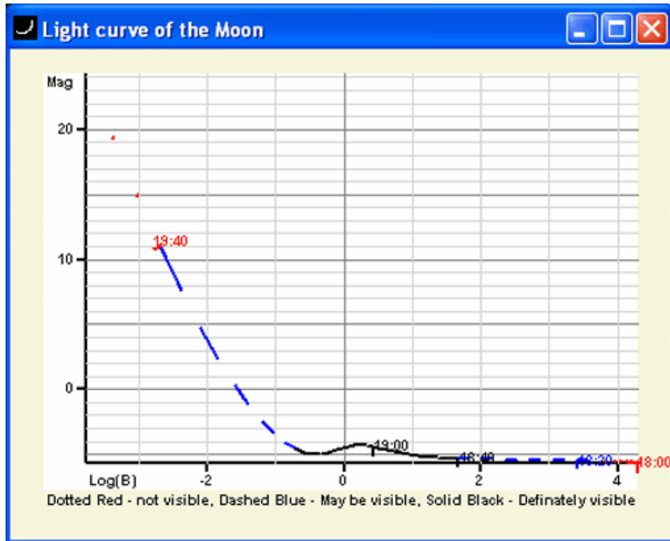
Figure 11. Light curve plot showing the magnitude against sky illuminance.
