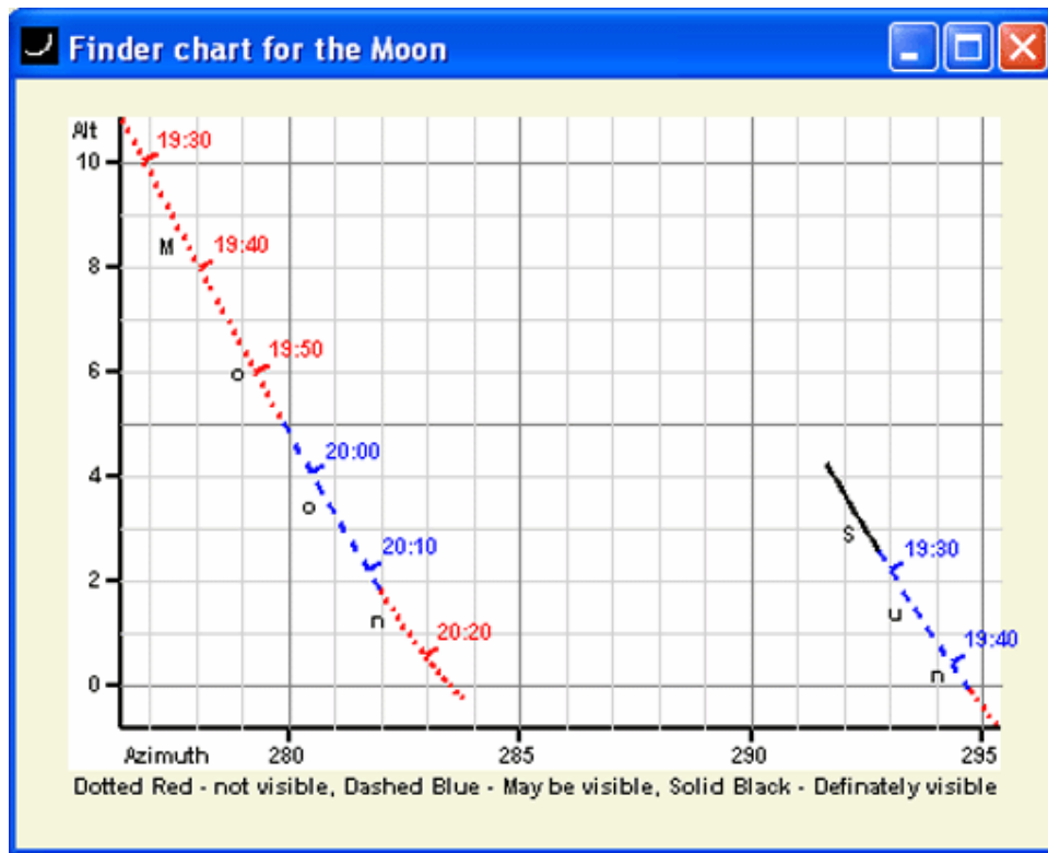
Figure 2. Finder chart showing the predicted appearance of the Moon adjusted for Roy Hoffman's eyesight. The period of visibility is reduced by a few minutes.
