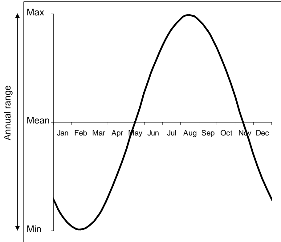
Figure 4. The annual (yearly) variation of a weather parameter ( Temperature, Pressure and Humidity )
