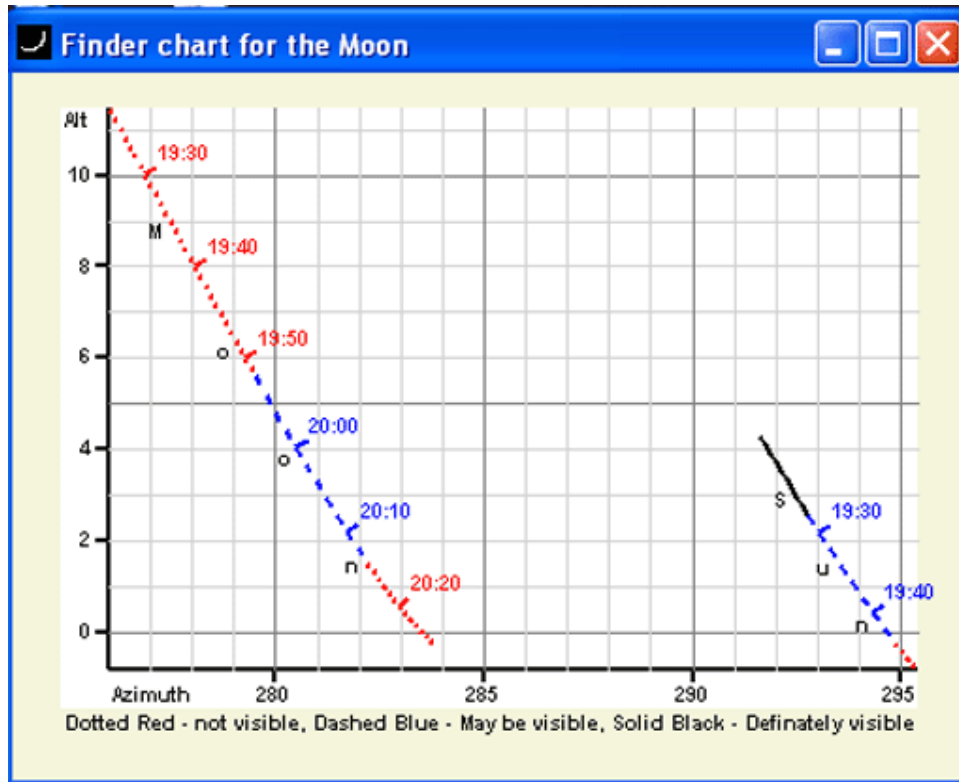
Figure 1. Finder chart showing the predicted appearance of the Moon.
