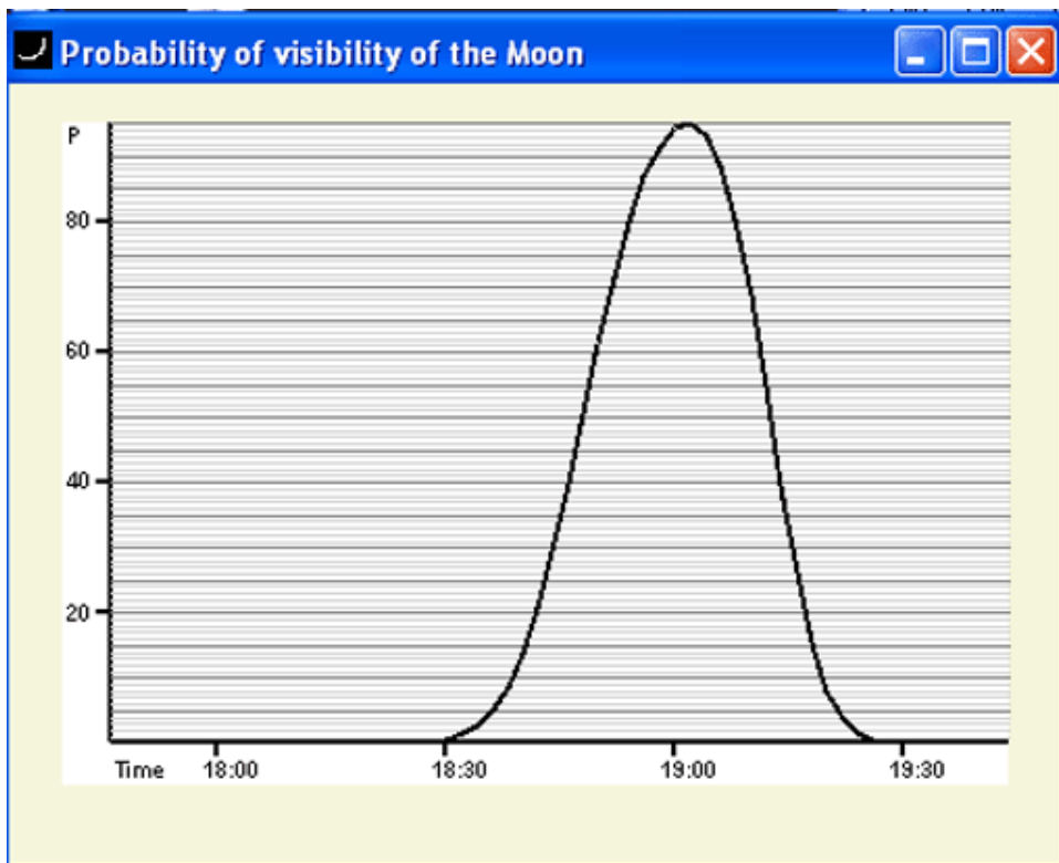
Figure 10. Probability plot showing the probability of naked eye visibility against time.
