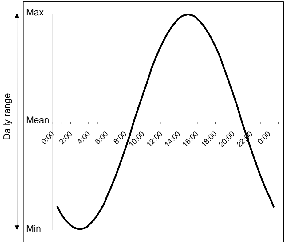
Figure 3. The daily (diurnal) variation of a weather parameter ( Temperature, Pressure and Humidity )
